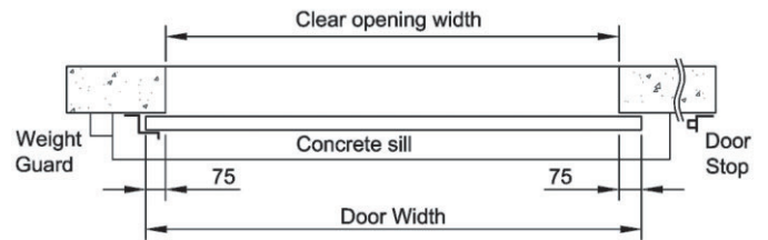
PLAN - WITH DOOR IN CLOSED POSITON
